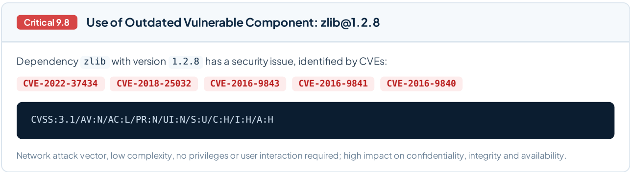
zlib@1.2.8 vulnerable dependency
